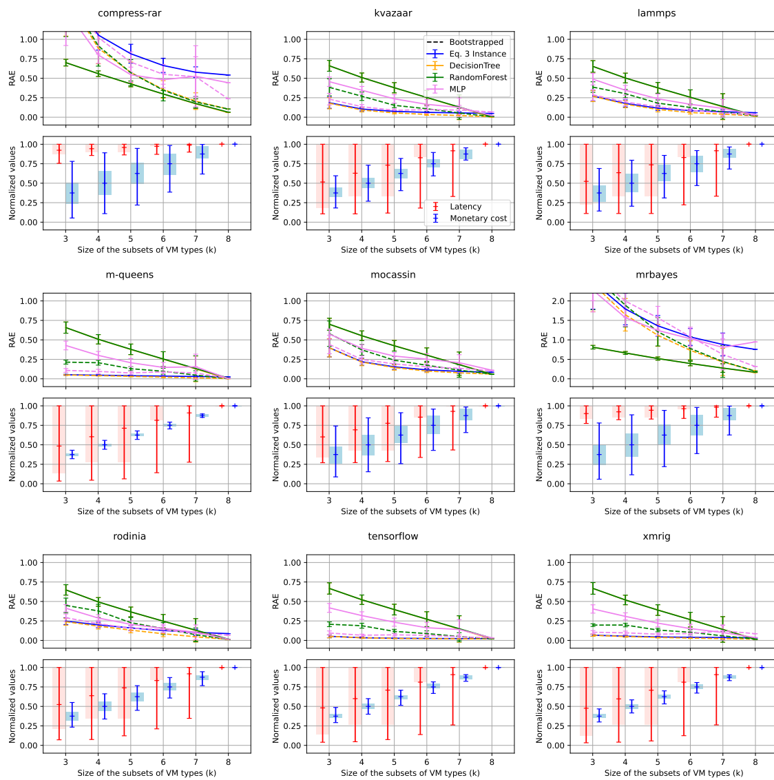
Fig. 4. Results with the M7i family for all benchmark applications
